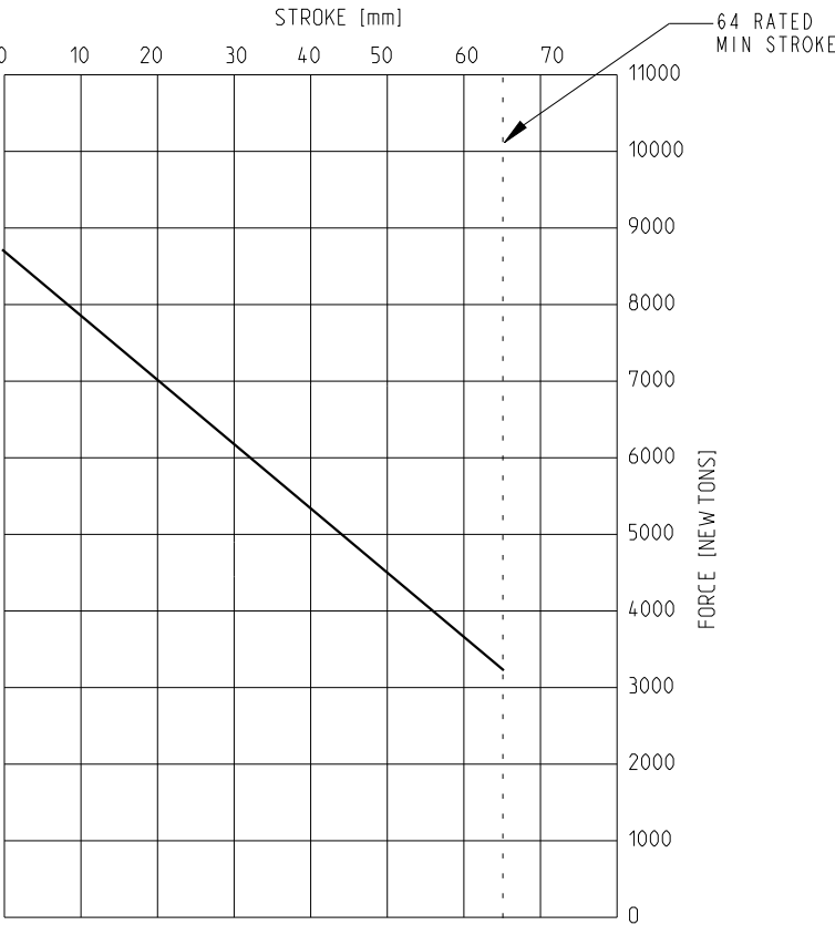
SPRING CHAMBER PERFORMANCE T-24 ACCORDING TO TÜV BC0176
