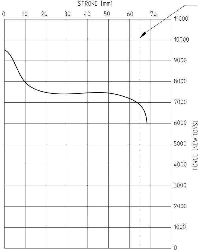
SERVICE CHAMBER PERFORMANCE T-20 ACCORDING TO TÜV BC 0176
