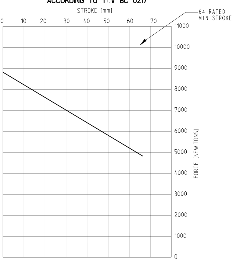
SPRING CHAMBER PERFORMANCE T-24 ACCORDING TO TÜV BC 0217
