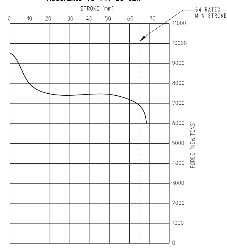
SERVICE CHAMBER PERFORMANCE T-20 6,5BAR ACCORDING TO TÜV BC 0217
