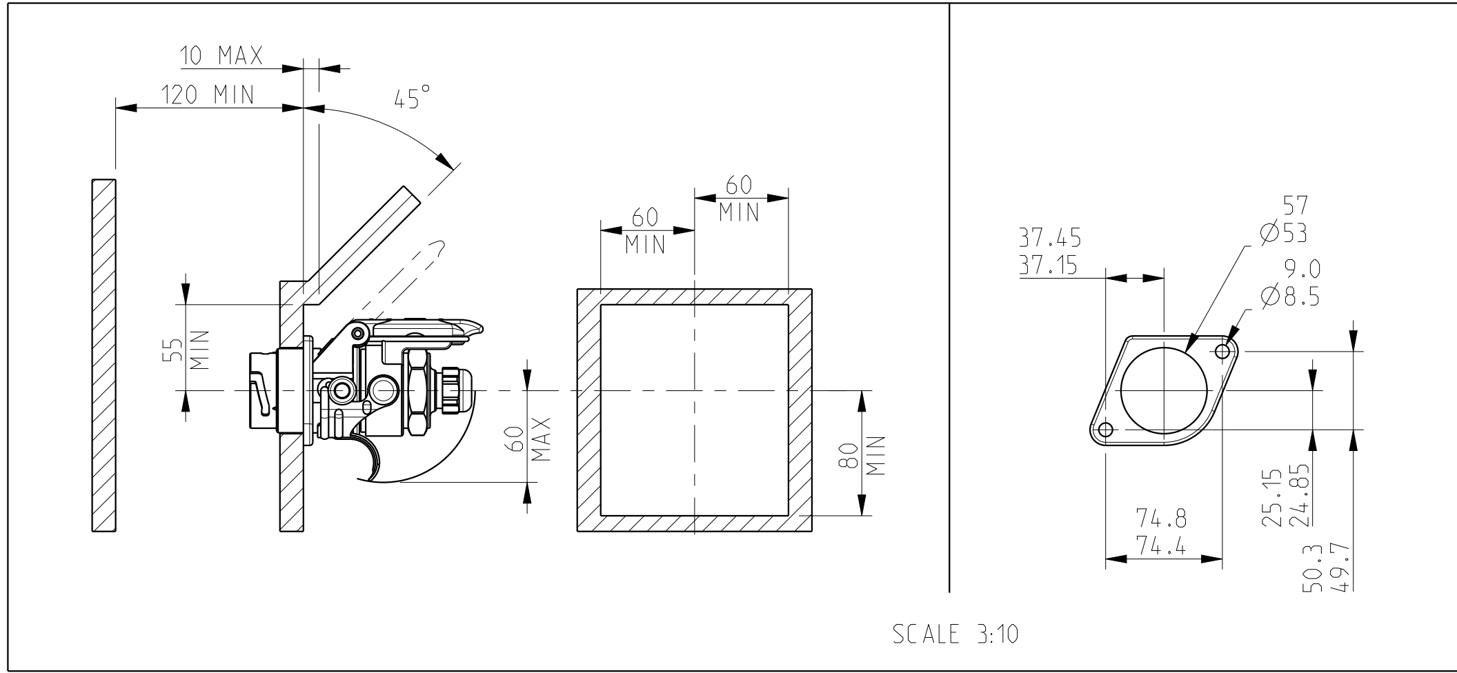
CLEARANCE DIMENSIONS
