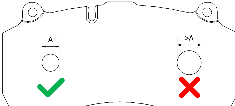
Fig. 1: A brake pad for the ModulT air disc brake is shown above. In the brake pad, the standard hole size is depicted to the left, and the enlarged hole is shown to the right.
