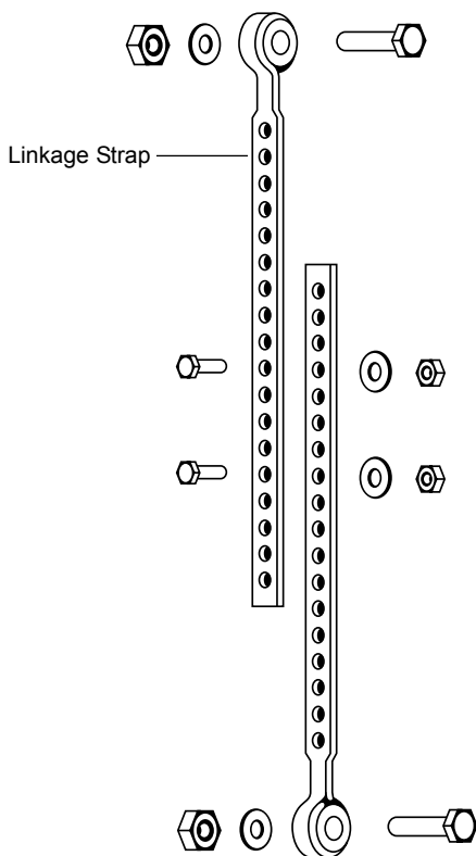
Figure 1. Adjustable Strap Linkage Exploded View
